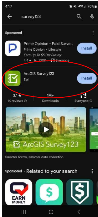
Screenshot 1.1
