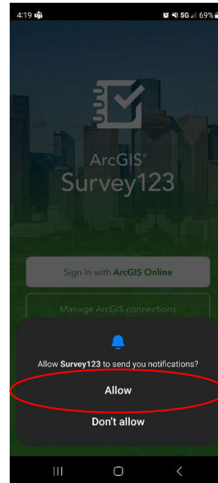
Screenshot 1.3
