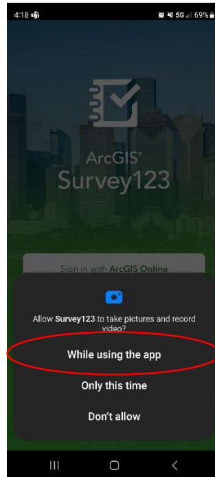
Screenshot 1.2
